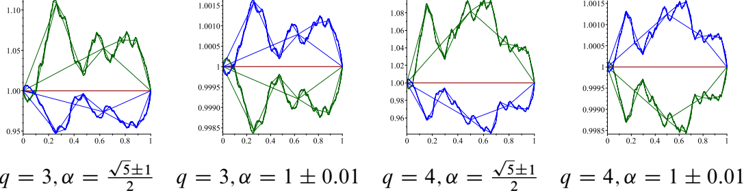
Figure 11: Periodic fluctuations of f(n)n^{-\log_q(1+(q-1)\alpha)} in the cases of nonzero digits of q -ary Gray codes for q = 3, 4 and different \alpha (Section 7.2).
